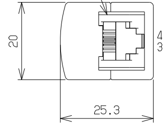
MJ2 (6極2心)
